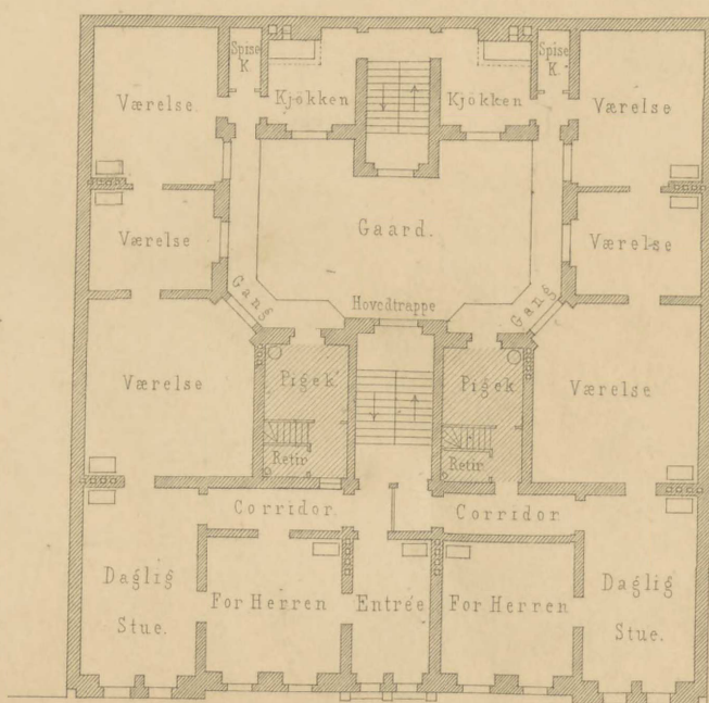
1 re ETAGE.
