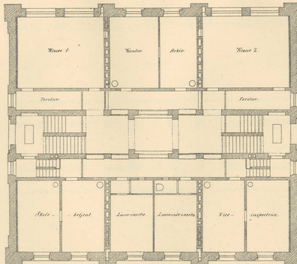
Plan of Stuen.
