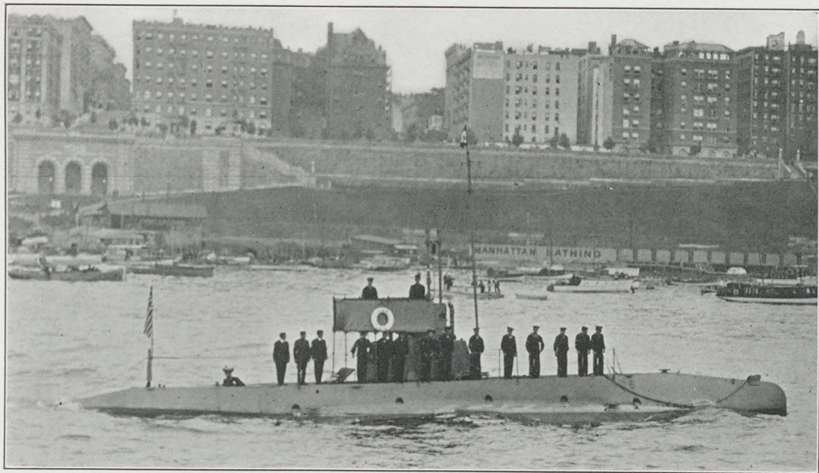
U.S. Submarine Torpedo Boat C-5
