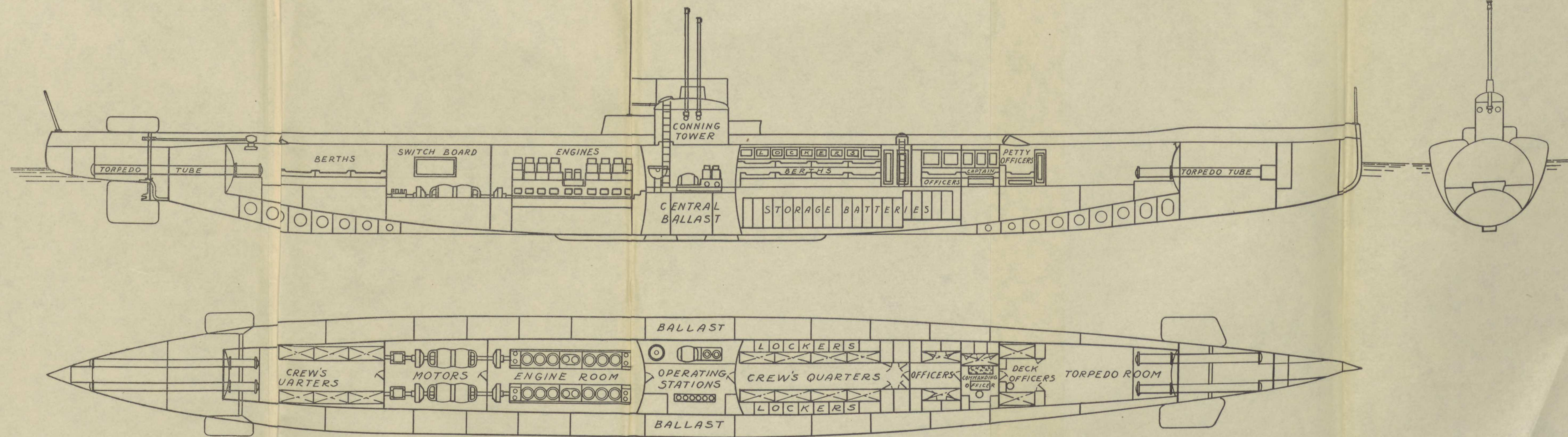
PLATE IV. PLAN AND PROFILE OF 600-TON LAURENTI SUBMARINE
