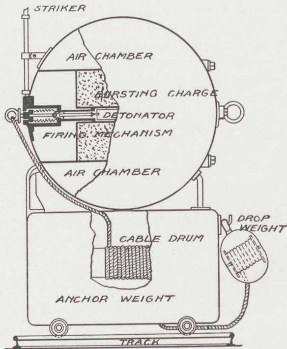
Simple contact mine
