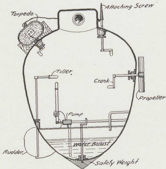
Bushnell's "Turtle." 1776
