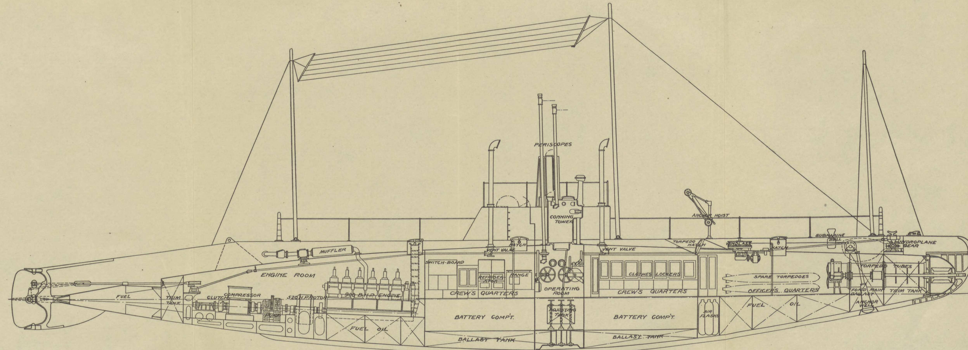
PLATE VI. PROFILE OF 830-TON ELECTRIC BOAT TYPE SUBMARINE
