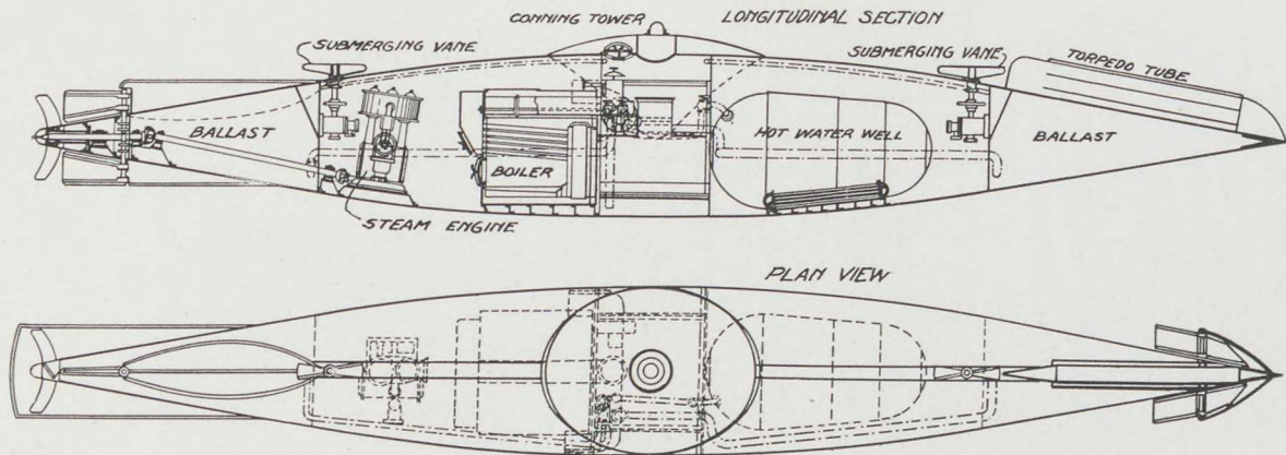
Nordenfelt's Turkish Submarine. 1887
