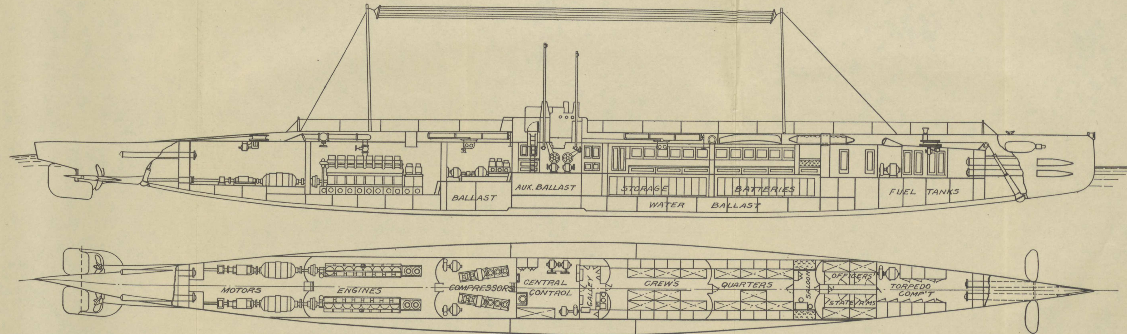
PLATE V. PLAN AND PROFILE OF 800-TON GERMAN SUBMARINE
