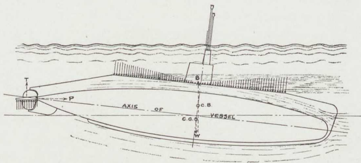
Figure 2. Diving Boat
