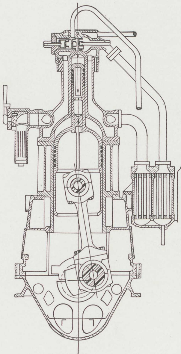
Section through air compressor
