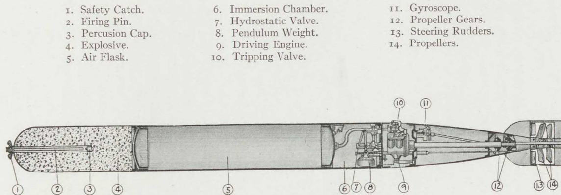
Cross-section through a modern automobile torpedo
