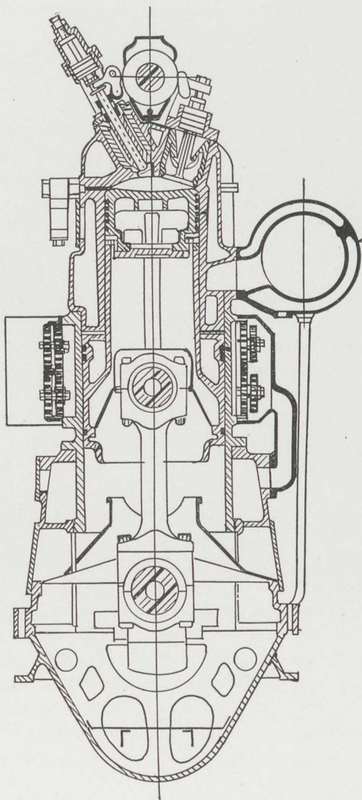
Section through working cylinder
