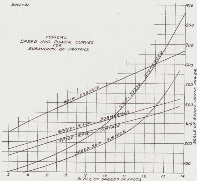
Plate II. Speed and Power Curves
