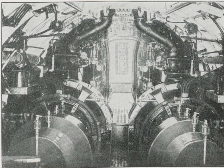
Main Motors, Submarine G-I. Main engines in background, forward of motors
