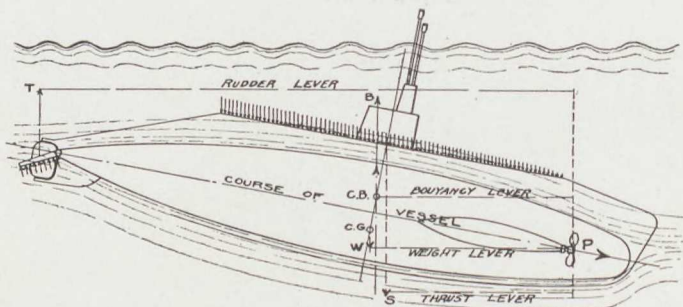
Figure 4. Forward Propulsion
