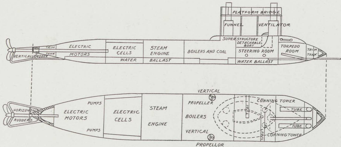
Hovgaard's Submersible
