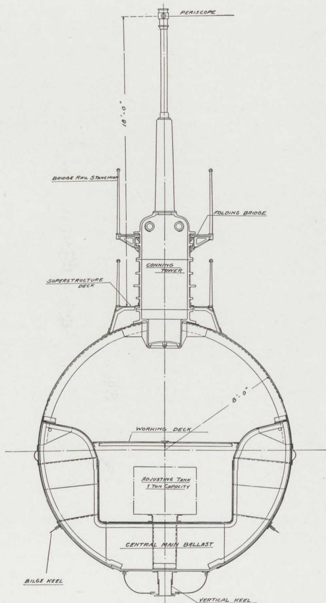
Midship Section, Electric Boat Co. Type
