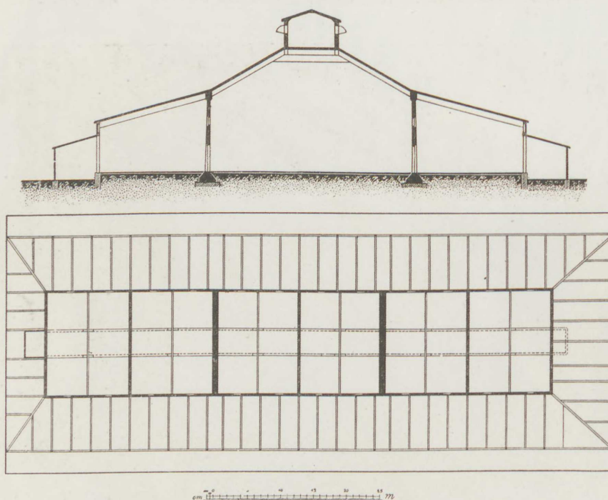
CEMENTSILO I AALBORG
