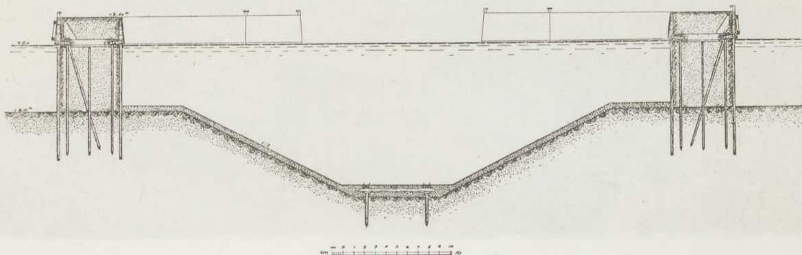
Snit A 4 -A 4
