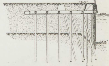
Snit A 3 -A 3
